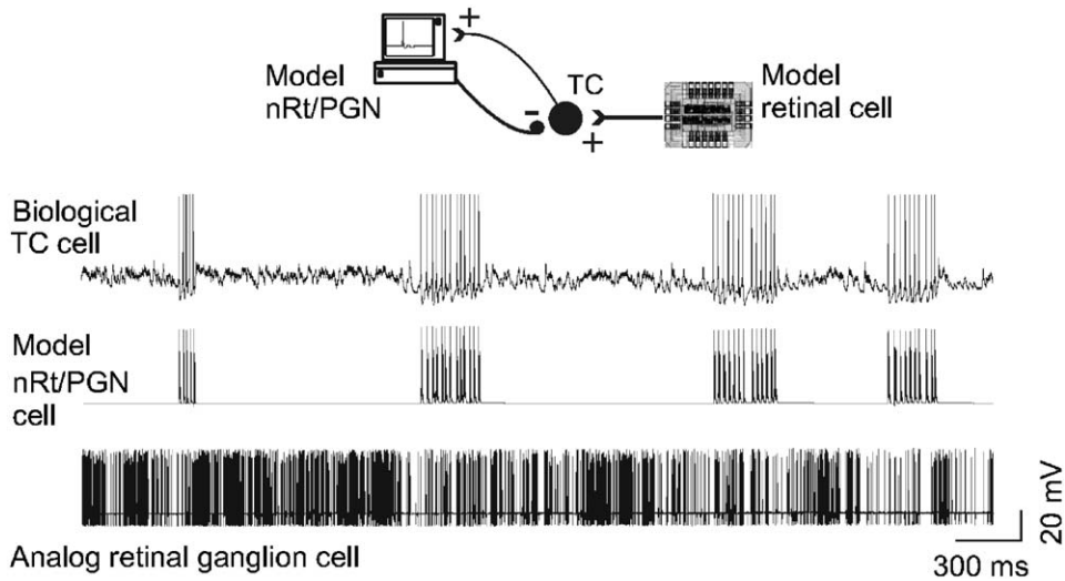
Fig. 4. Emergent rhythmic activity in a hybrid circuit mixing model and biological neurons. An analog model neuron (bottom trace) was programmed to simulate the temporal structure of real retinal cell discharges and the kinetics of real AMPA receptor-mediated excitatory postsynaptic potentials (EPSPs). Hybrid thalamic circuits receiving this emulated synaptic bombardment spontaneously generated short epochs of oscillation, recurring periodically in a manner very similar to biological spindle waves occurring in sleep.
