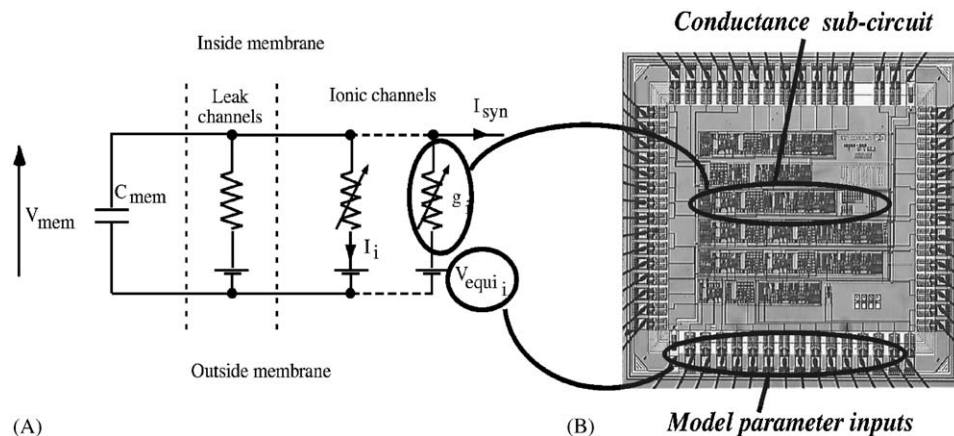
Fig. 1. (A) Electrical equivalent circuit of excitable membrane, following Hodgkin–Huxley formalism, (B) Microphotograph of an analog conductance-based ASIC (technology: AMS BiCMOS 0.8 \mu\text{m} , chip area: 4 \times 4 \text{mm}^2 ); input pads receive voltages to set the model parameters: one silicon row corresponds to one conductance sub-circuit.
