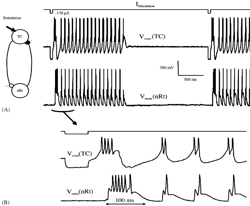
Fig. 3. (A) When a negative current pulse is injected into a TC biological neuron the characteristic response is a rebound burst of action potential. The simulation reproduces the same pattern. When two neurons TC and nRt are synaptically coupled by an inhibitory (nRt \rightarrow TC) and an excitatory synapse (TC \rightarrow nRt) the same inhibitory pulse generates a sustained oscillation until a relaxing state occurs [5], (B) Zoom of plot A. One can observe precisely the individual action potential shape.
