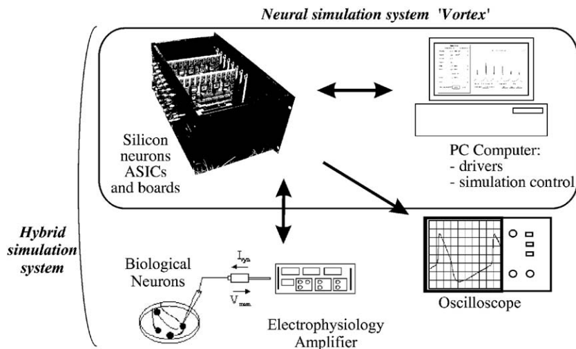
Fig. 2. The Vortex simulation platform with peripherals. The system is organized around a rack containing the artificial neurons chips. The control software runs on a PC. To run hybrid networks experiments, artificial neurons are connected to biological neurons via an electrophysiology amplifier.
