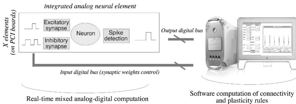
Fig. 5. Hardware/software structure of the mixed analog–digital simulation system. Neural elements are analog integrated circuits, on electronics boards ( X neural elements per board, X depending on the ASIC version). A PCI interface allows digital transfer between the circuits and a custom software. A real-time software/hardware closed-loop processes the neuronal spikes and dynamically controls synaptic quantum and connectivity updates.
